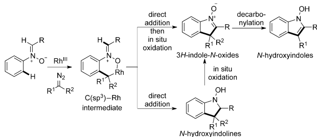
Scheme 2. Rhodium(III)-catalyzed C–H functionalization.
