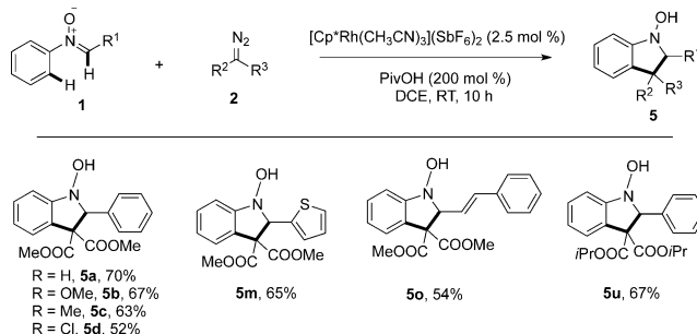
Scheme 5. Rhodium(III)-catalyzed synthesis of N -hydroxyindolines from nitrones and diazo compounds. Reactions were carried out on a 0.2 mmol scale. Yields of the isolated products are given.
